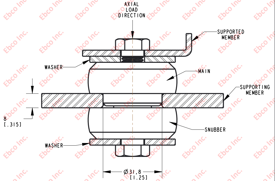
INSTALLATION VIEW (Shown under no load)
